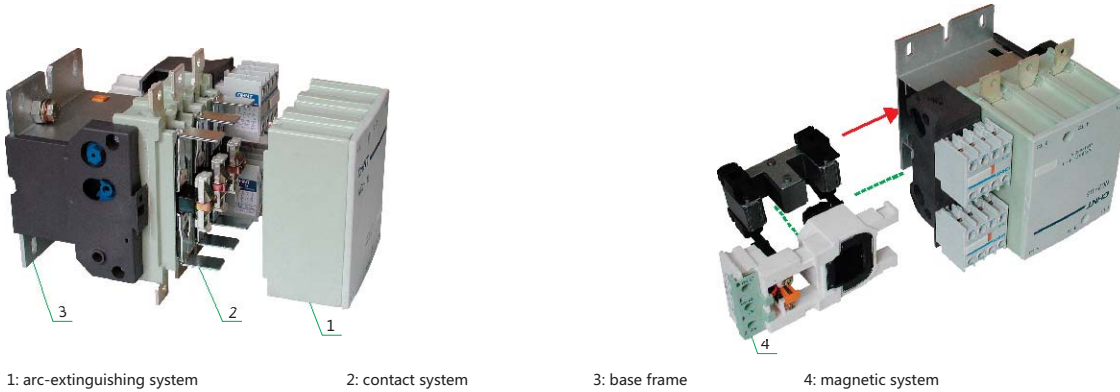
1: arc-extinguishing system 2: contact system 3: base frame 4: magnetic system
